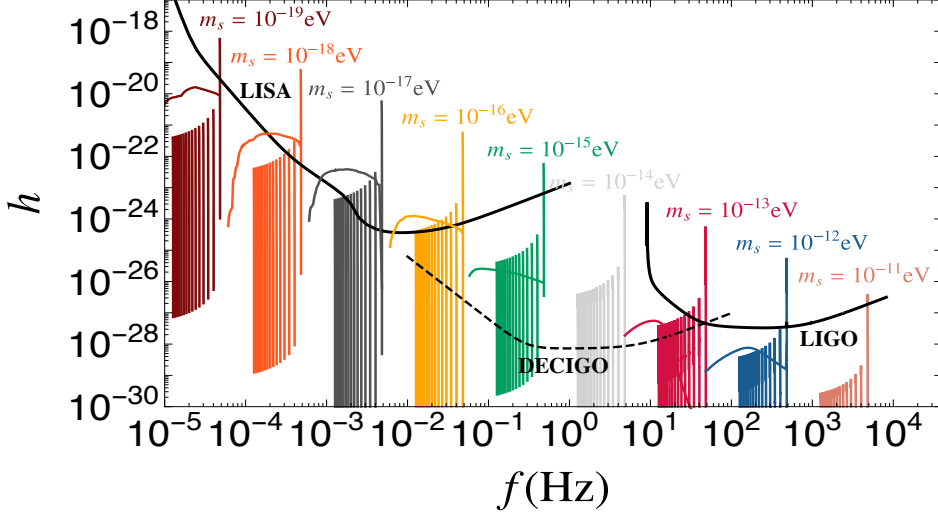
Figure 61: Root-mean-square GW strain produced by BH-scalar condensates compared to the Advanced LIGO PSD at design sensitivity [654] and to the non-sky averaged LISA PSD [637] (black thick curves), assuming a coherent observation time of T_{\text{obs}} = 4\text{yr} in both cases. Each (nearly vertical) line shows the strain for a given boson mass m_S , computed at redshift z \in (0.001, 3.001) (from right to left, in steps of \delta z = 0.2 ), with M\mu_S increasing in the superradiant range (0, M\Omega_H) along each line, and assuming an initial BH spin a = 0.9M . Different colors correspond to different boson masses m_S . Thin lines show the stochastic background produced by the whole population of astrophysical BHs under the optimistic assumptions of Ref. [127, 128]. The PSD of DECIGO [653] (dashed line) is also shown for reference. From [127]. Similar results (but with stronger signals) hold for the vector and tensor cases [472].
