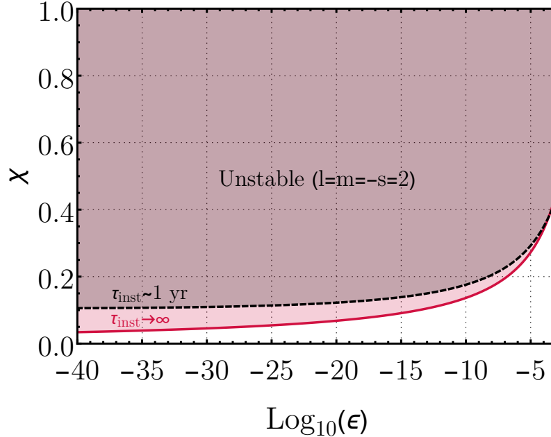
Figure 71: Exclusion plot in the \chi - \epsilon plane due to the ergoregion instability of a perfectly-reflecting ECO, assumed to be described by the Kerr geometry in their exterior, r > r_0 = r_+(1 + \epsilon) . Shaded areas represent regions where the object is unstable against l = m = 2 gravitational perturbations with a time scale equal to or shorter than \tau_{\text{inst}} . For details see Refs. [609, 698, 228].
