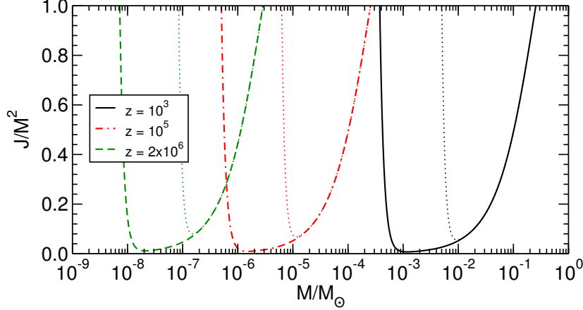
Figure 67: Contour plots in the BH Regge plane [9, 10, 105] corresponding to a plasma-triggered instability of a primordial BH whose time scale is shorter than the age of the universe at a given redshift, assuming a mean cosmic gas density (6.24). Thick and thin curves correspond to polar and axial modes, respectively [105]. In both families, the rightmost part of each curve is described by J/M^2 \sim 4M\omega_p . Roughly speaking, primordial BHs in the mass range 7 \times 10^{-9} M_\odot < M < 0.2 M_\odot go through a cosmic era (at some redshift 10^3 < z < 2 \times 10^6 ) when the superradiant instability is effective. From [530].
