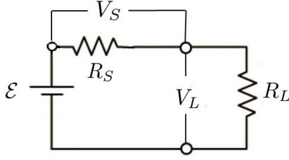
Figure 74: Circuit analogy of the BZ mechanism in which a battery transfers energy to a load. A battery of electromotive force \mathcal{E} with internal resistance R_S drives a current I through the load resistance R_L (which could be for example an electric light). Maximum power transfer is attained when R_L = R_S .
