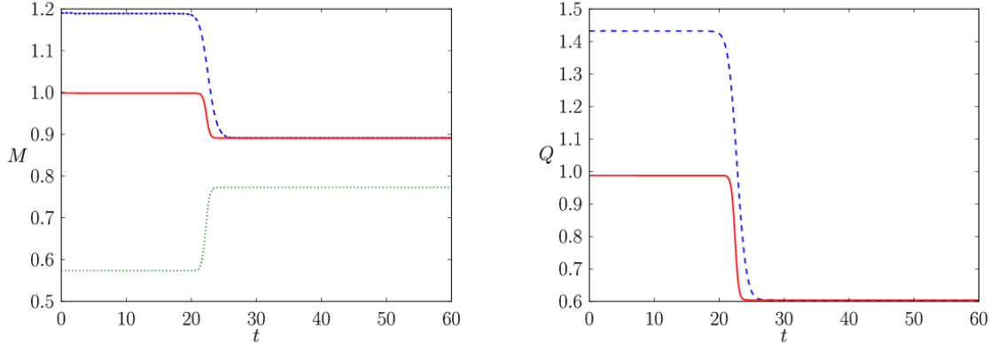
Figure 12: Time evolution of the BH mass and charge for the superradiant scattering of a massless scalar field around a BH with initial charge Q = 0.987M . The charge of the scalar field and the initial data for the simulation are chosen in such a way that one expects superradiant scattering to occur. Left: Evolution of the BH mass (solid red), Bondi mass (dashed blue) and irreducible mass (dotted green). Right: Evolution of the BH charge at the horizon (solid red) and total charge measured at future null infinity (dashed blue). From [235].
