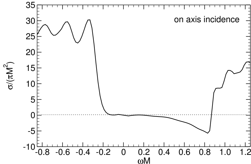
Figure 16: Absorption cross-section of a gravitational plane wave incident on a rotating Kerr BH ( a/M = 0.99 ) along the rotation axis. The figure shows that counter-rotating ( \omega < 0 ) plane waves are more absorbed than co-rotating waves ( \omega > 0 ), and that in the superradiant regime plane waves are amplified.
