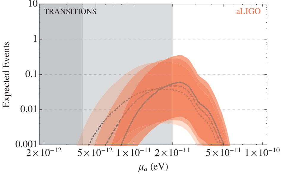
Figure 63: Expected number of events for GWs emitted thorough level transitions with aLIGO at design sensitivity [611] as a function of the axion mass (but the results are also valid for a generic scalar field). The vertical shaded regions are disfavored by BH spin measurements assuming the QCD axion coupling strength (light gray) or stronger (dark grey). For stronger axion couplings nonlinear effects become important and extrapolations of the linearized results are not reliable (cf. Sec. 5.8). Each of the three bands corresponds to varying the BH mass distribution width including optimistic and pessimistic estimates of astrophysical uncertainties. See Ref. [103] for details.
