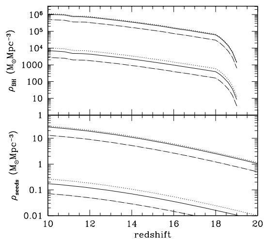
Figure 2. Lower panel: comoving density of 20 M_{\odot} black hole seeds as a function of redshift. Upper panel: comoving density of black holes, assuming continuous formation and growth of seeds to 10^6 M_{\odot} according to equation (13), starting from z = 20 . Solid line: Mestel disc, dotted line: rigid disc, dot–dashed line: exponential disc. The upper set of lines assumes f_d = 0.5 , the lower set assumes f_d = 0.1 .
